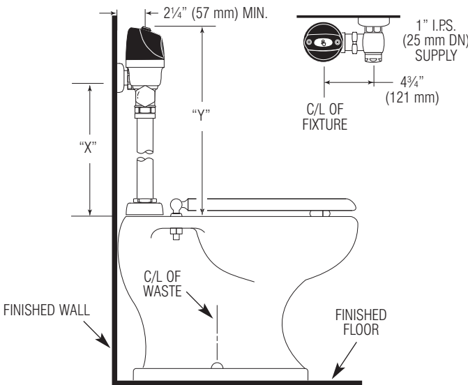
High Rough-in Water Closet Installation Models 8113, 8115 & 8116
